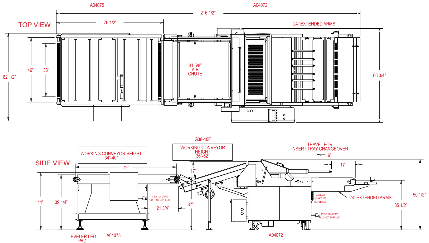
Typical Layout For Spreader Belt System
